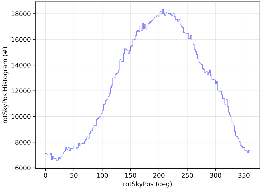
roll_uniform_early_half_mjdp0_v3.4_10yrs WFD all bands: rotSkyPos Histogram
