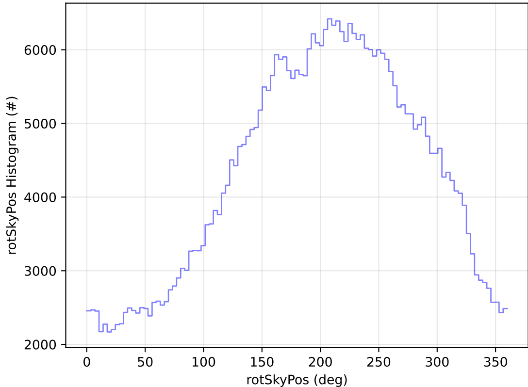
roll_uniform_early_half_mjdp0_v3.4_10yrs All sky z band: rotSkyPos Histogram
