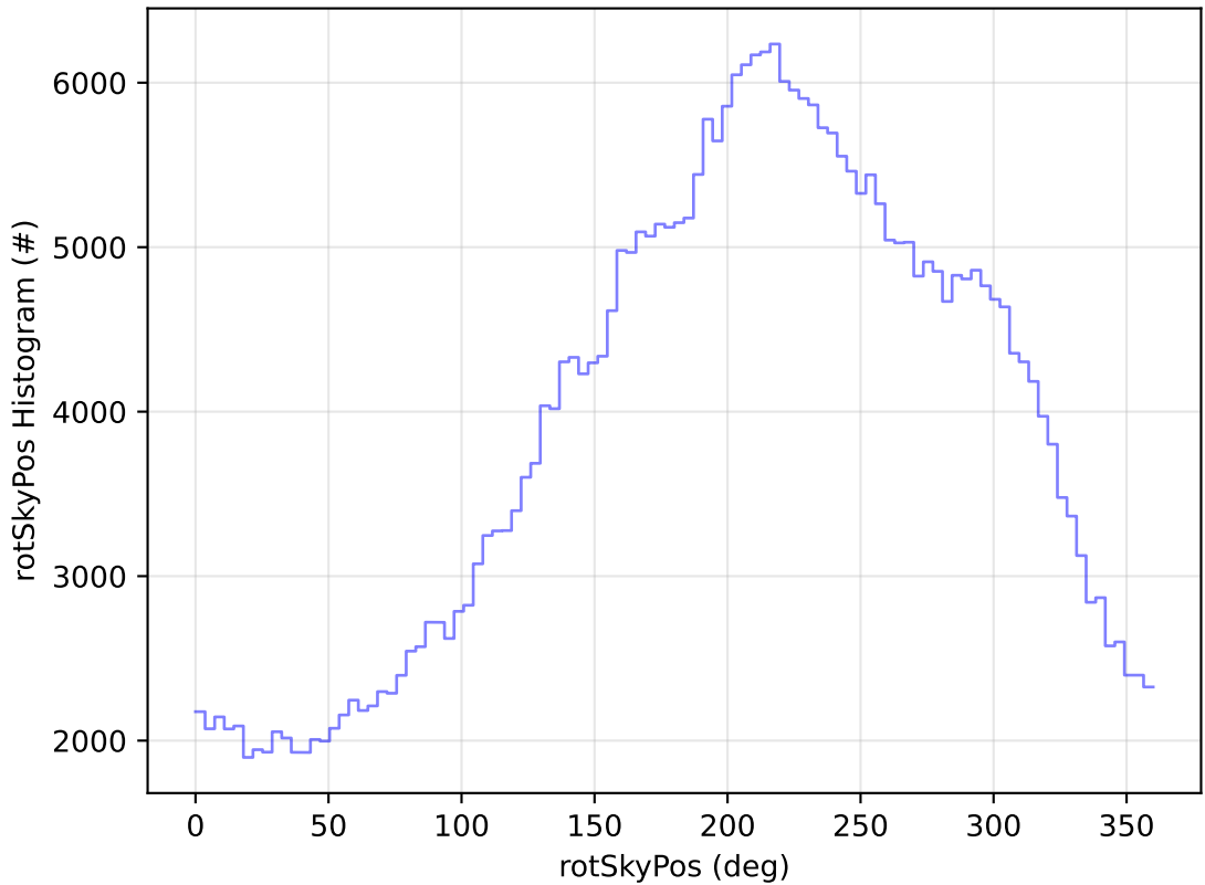
roll_uniform_early_half_mjdp0_v3.4_10yrs All sky y band: rotSkyPos Histogram
