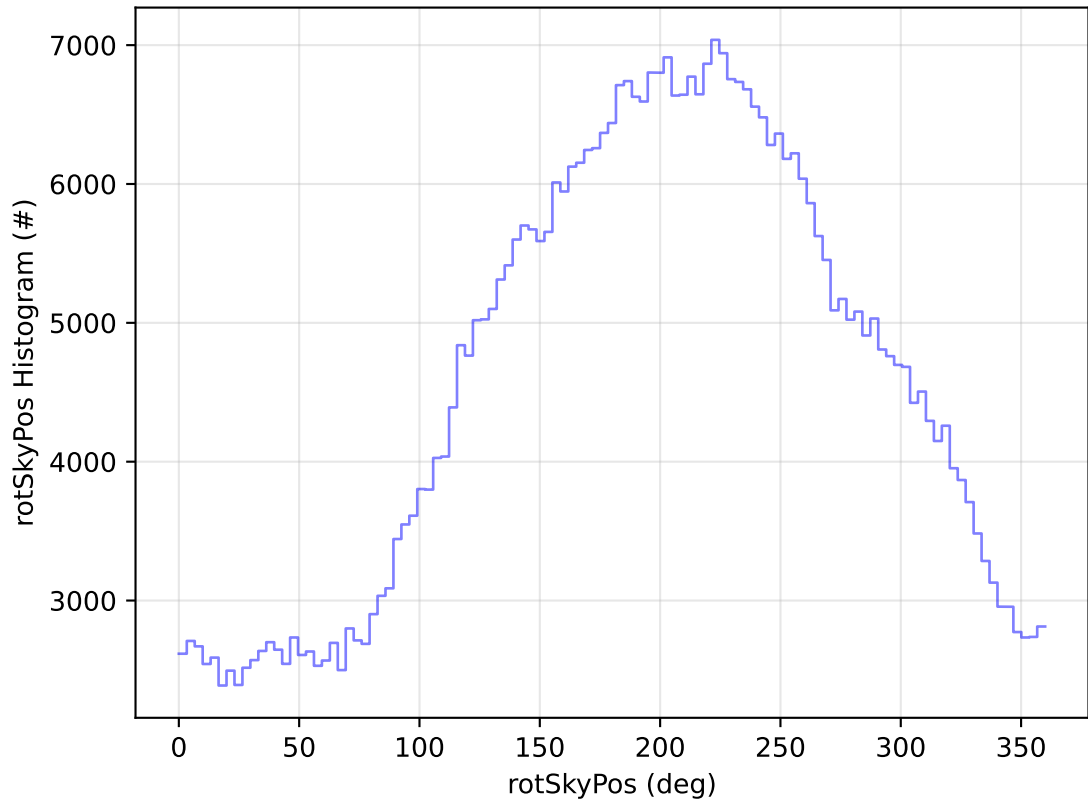
roll_uniform_early_half_mjdp0_v3.4_10yrs All sky i band: rotSkyPos Histogram
