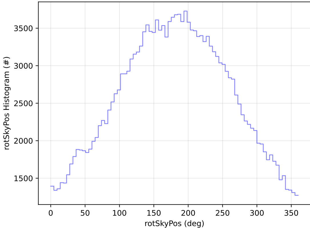
roll_uniform_early_half_mjdp0_v3.4_10yrs All sky g band: rotSkyPos Histogram
