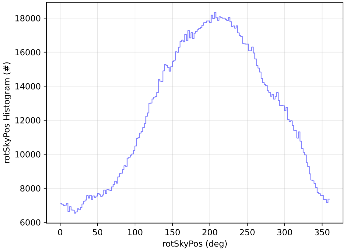
roll_uniform_early_half_mjdp0_v3.4_10yrs All sky all bands: rotSkyPos Histogram
