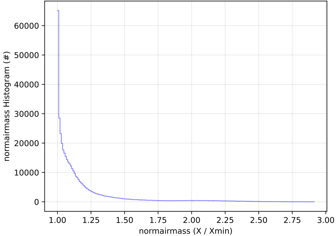
roll_uniform_early_half_mjdp0_v3.4_10yrs WFD z band: normairmass Histogram
