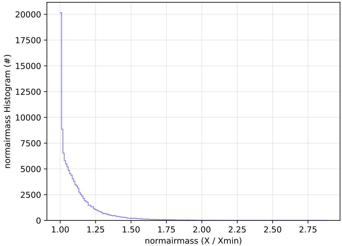
roll_uniform_early_half_mjdp0_v3.4_10yrs WFD u band: normairmass Histogram
