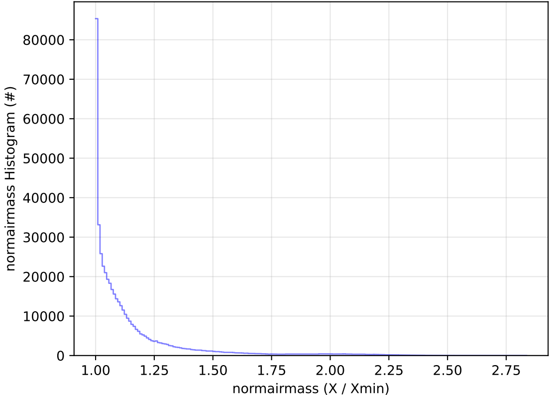
roll_uniform_early_half_mjdp0_v3.4_10yrs WFD r band: normairmass Histogram
