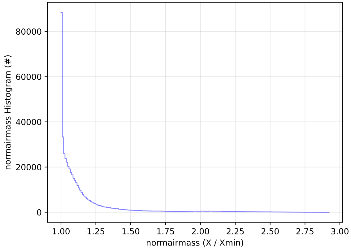
roll_uniform_early_half_mjdp0_v3.4_10yrs WFD i band: normairmass Histogram
