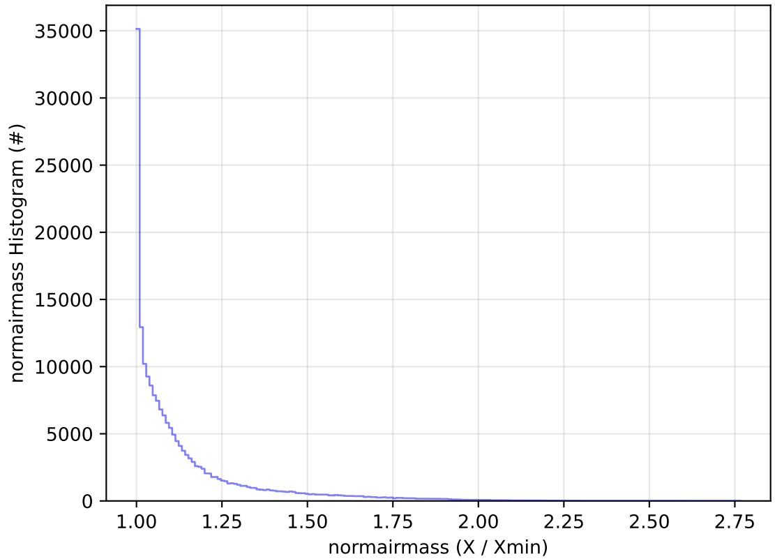
roll_uniform_early_half_mjdp0_v3.4_10yrs WFD g band: normairmass Histogram
