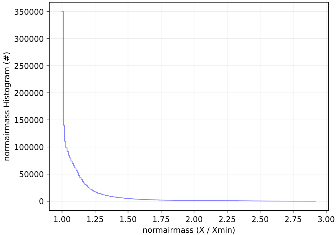
roll_uniform_early_half_mjdp0_v3.4_10yrs WFD all bands: normairmass Histogram
