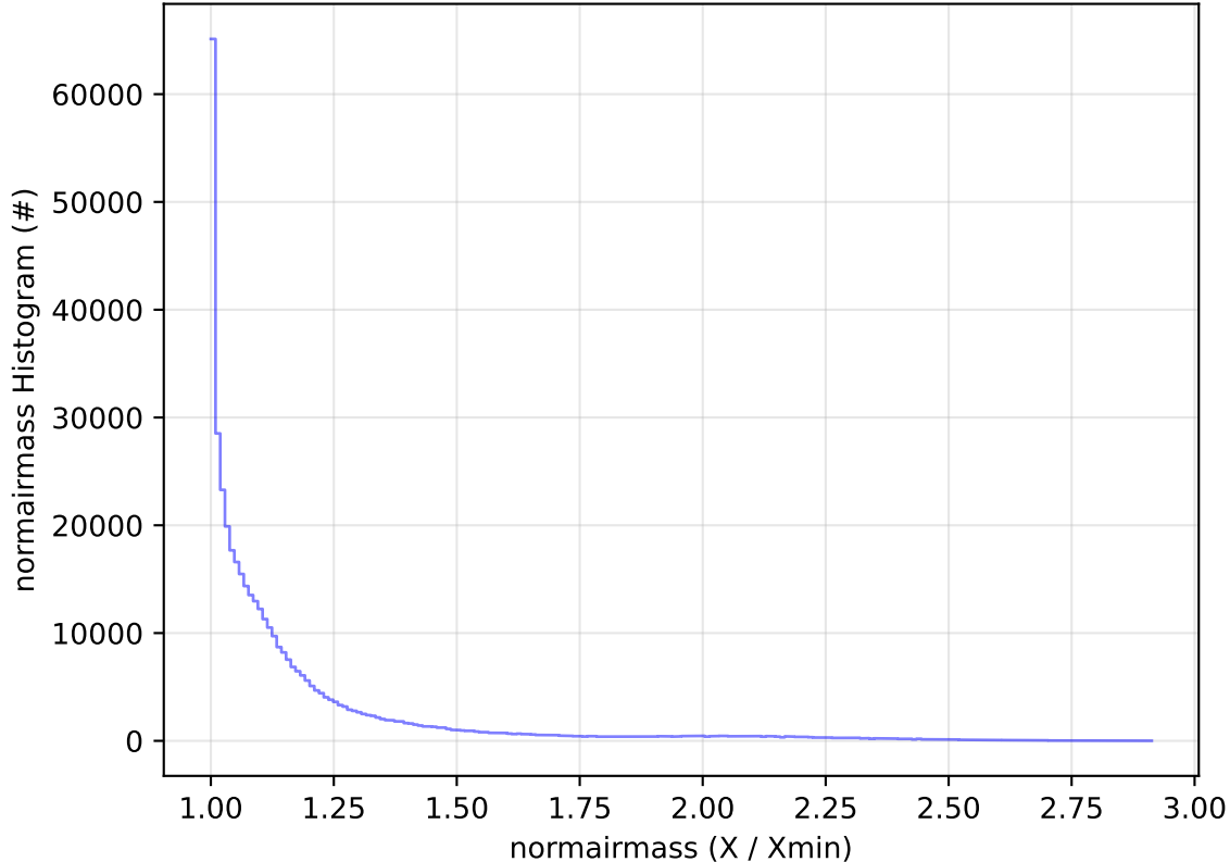
roll_uniform_early_half_mjdp0_v3.4_10yrs All sky z band: normairmass Histogram
