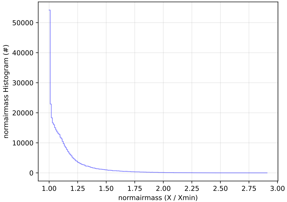
roll_uniform_early_half_mjdp0_v3.4_10yrs All sky y band: normairmass Histogram
