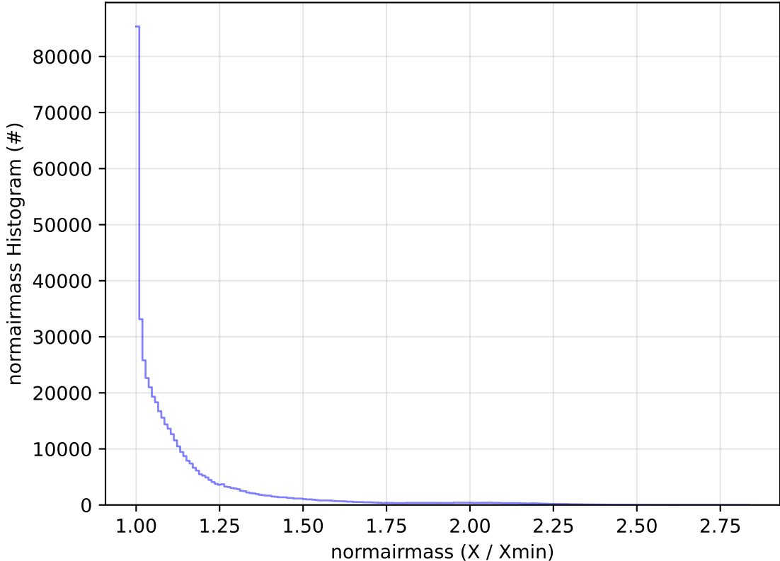
roll_uniform_early_half_mjdp0_v3.4_10yrs All sky r band: normairmass Histogram
