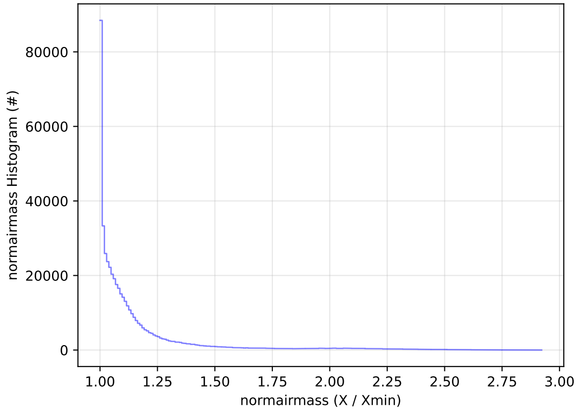
roll_uniform_early_half_mjdp0_v3.4_10yrs All sky i band: normairmass Histogram
