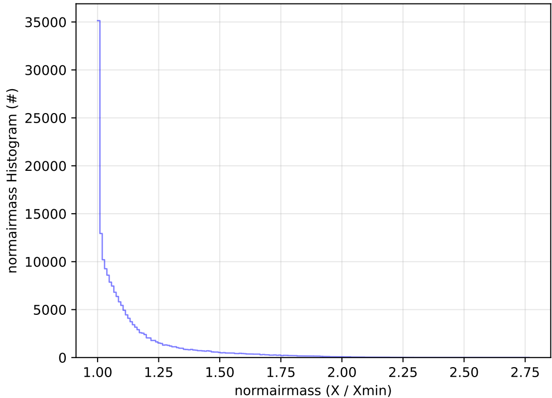
roll_uniform_early_half_mjdp0_v3.4_10yrs All sky g band: normairmass Histogram
