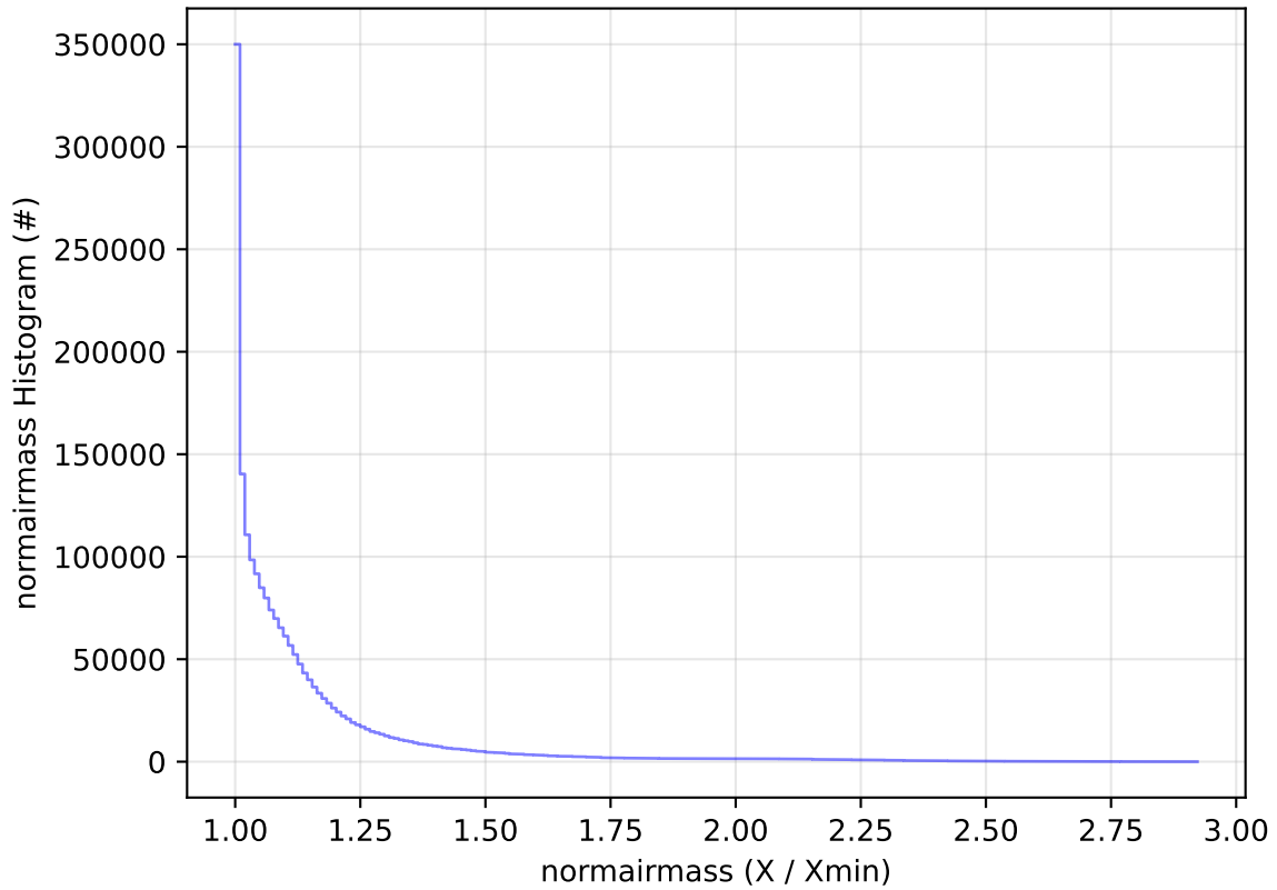
roll_uniform_early_half_mjdp0_v3.4_10yrs All sky all bands: normairmass Histogram
