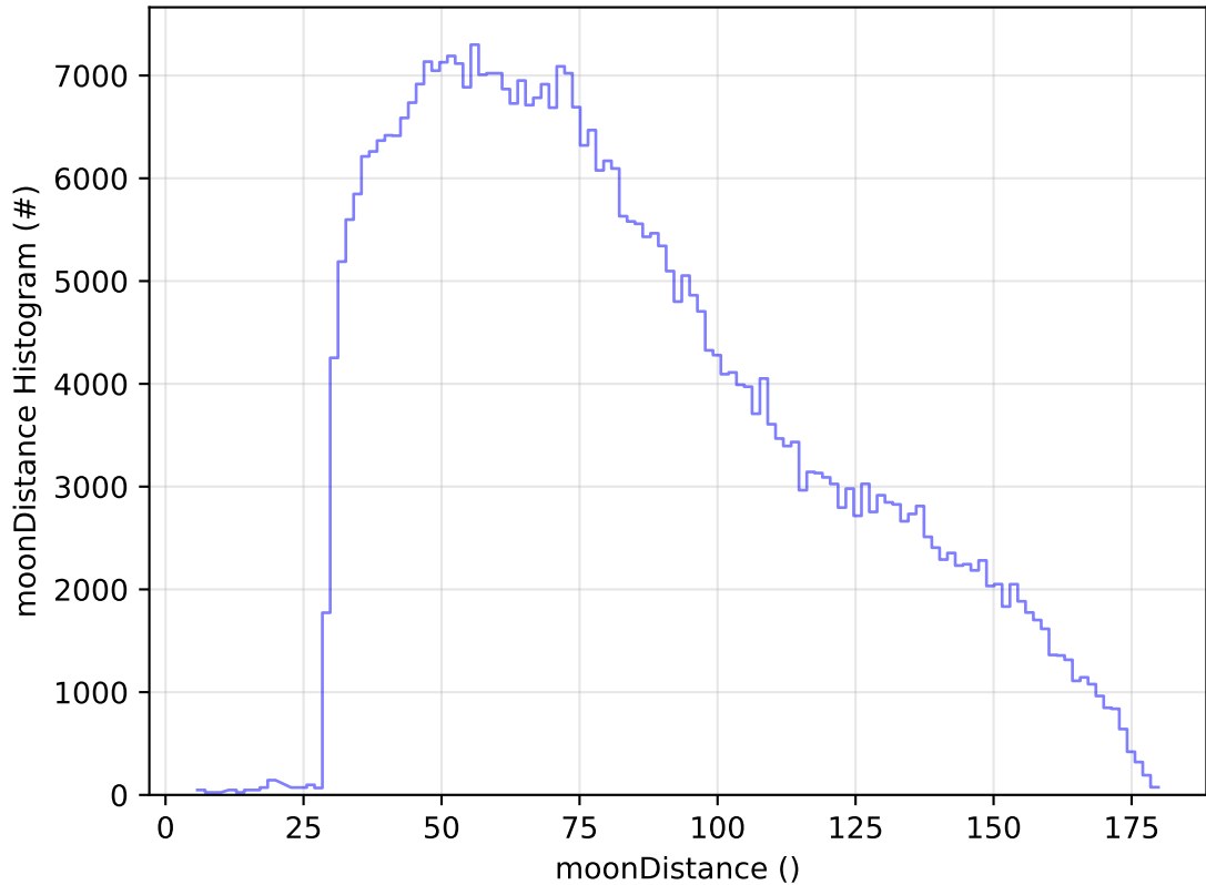
roll_uniform_early_half_mjdp0_v3.4_10yrs WFD z band: moonDistance Histogram
