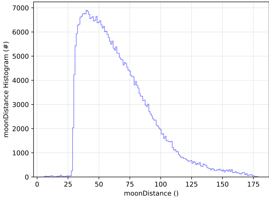
roll_uniform_early_half_mjdp0_v3.4_10yrs WFD y band: moonDistance Histogram
