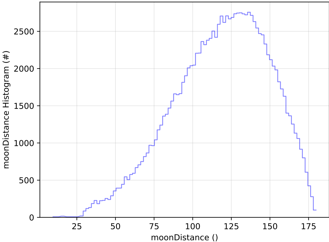
roll_uniform_early_half_mjdp0_v3.4_10yrs WFD u band: moonDistance Histogram
