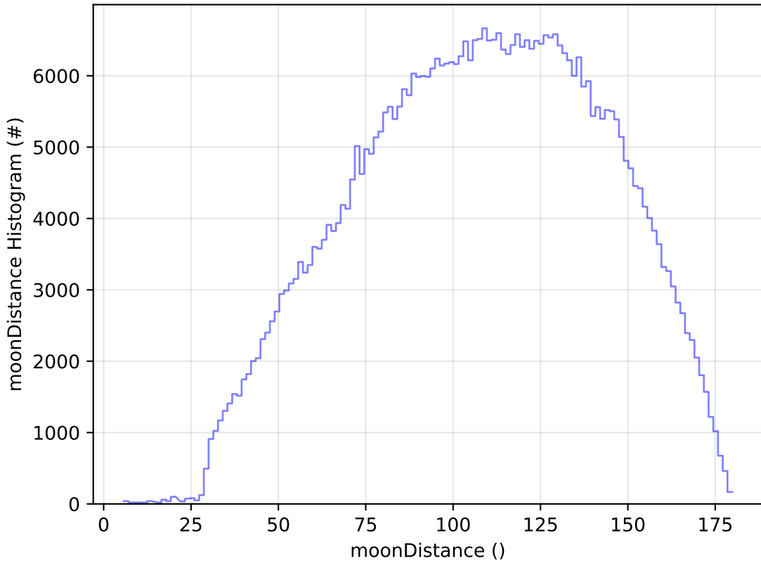
roll_uniform_early_half_mjdp0_v3.4_10yrs WFD r band: moonDistance Histogram
