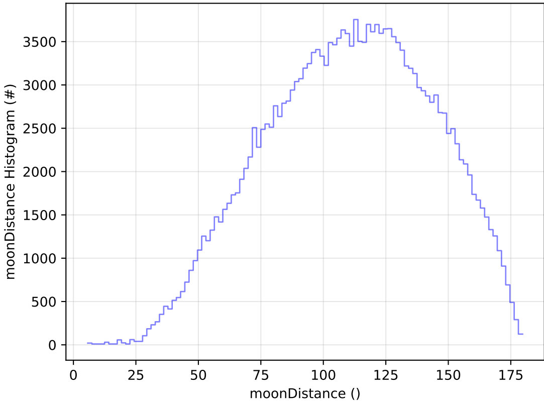
roll_uniform_early_half_mjdp0_v3.4_10yrs WFD g band: moonDistance Histogram
