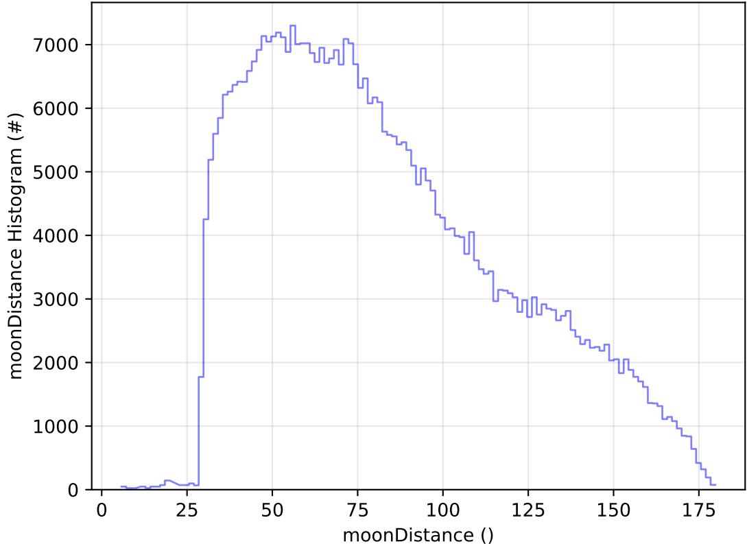
roll_uniform_early_half_mjdp0_v3.4_10yrs All sky z band: moonDistance Histogram
