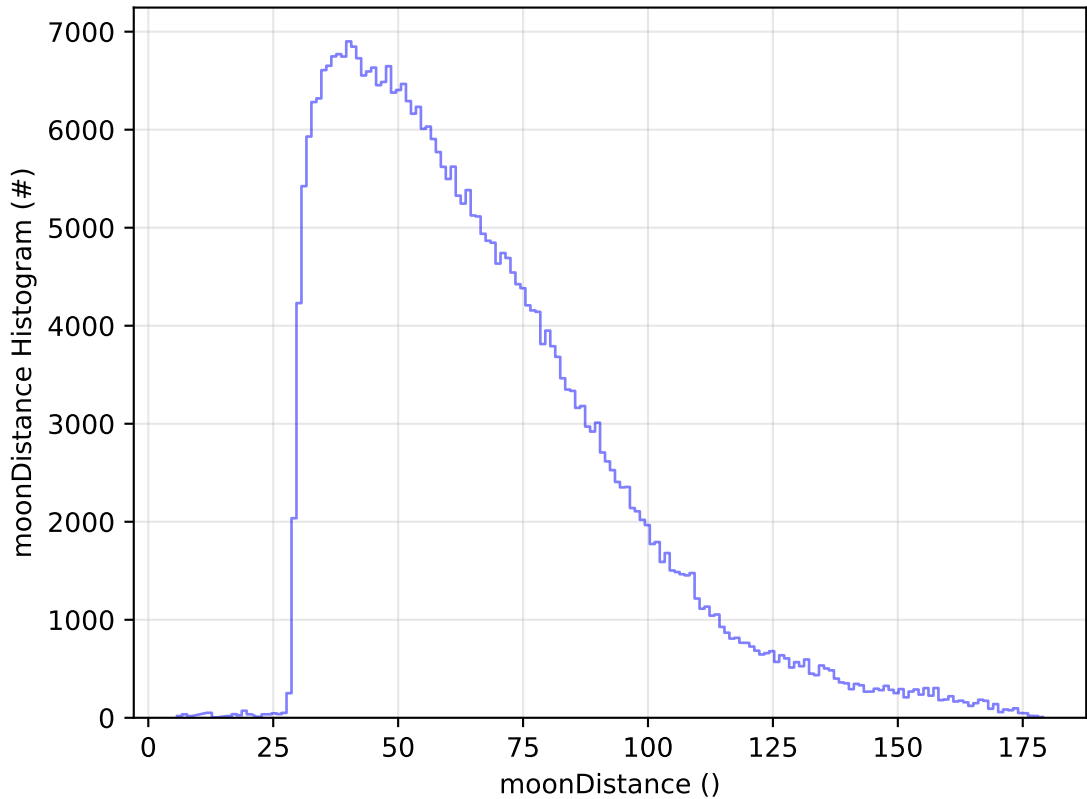
roll_uniform_early_half_mjdp0_v3.4_10yrs All sky y band: moonDistance Histogram
