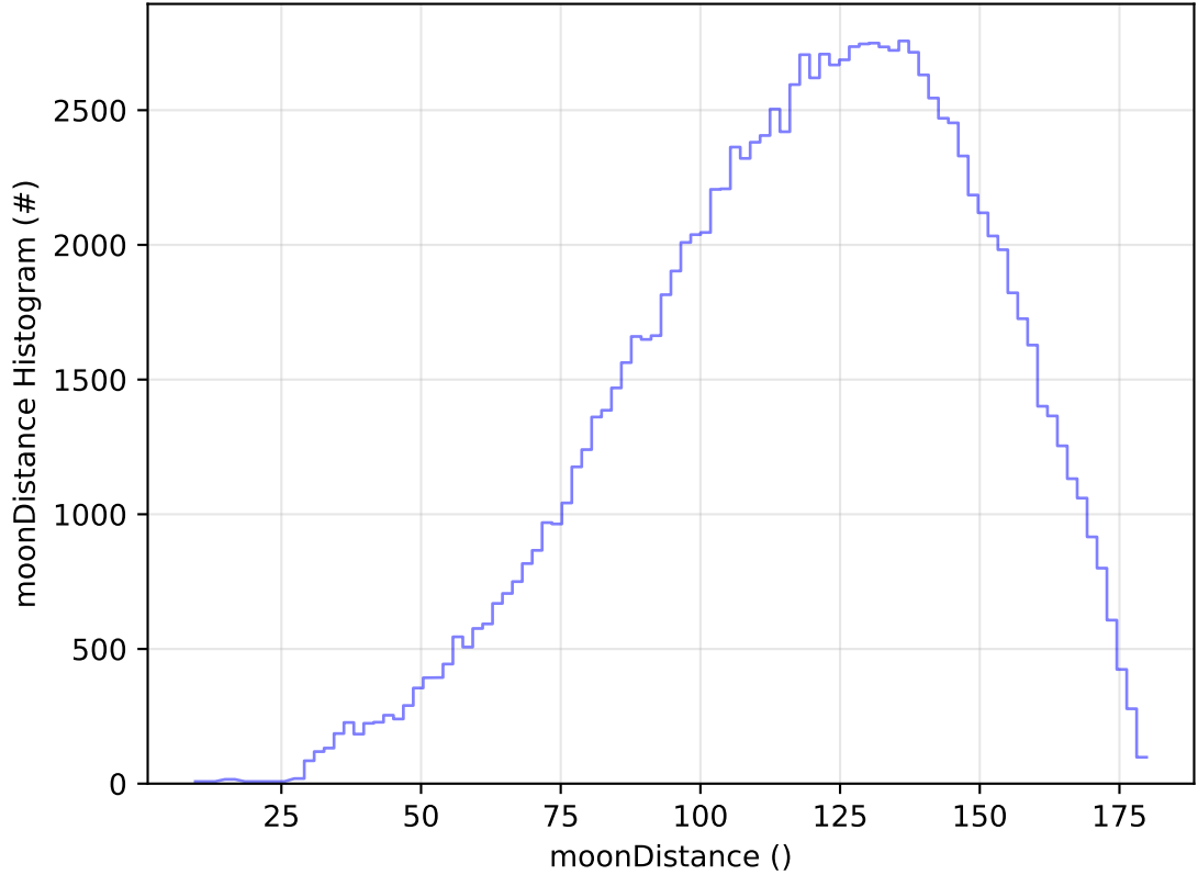
roll_uniform_early_half_mjdp0_v3.4_10yrs All sky u band: moonDistance Histogram
