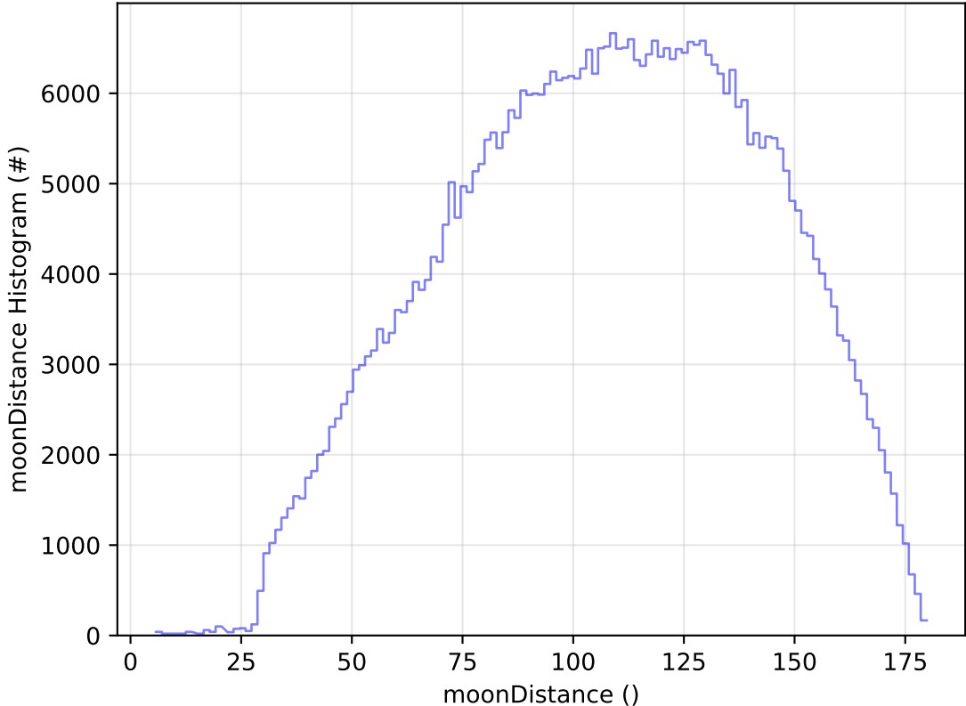
roll_uniform_early_half_mjdp0_v3.4_10yrs All sky r band: moonDistance Histogram
