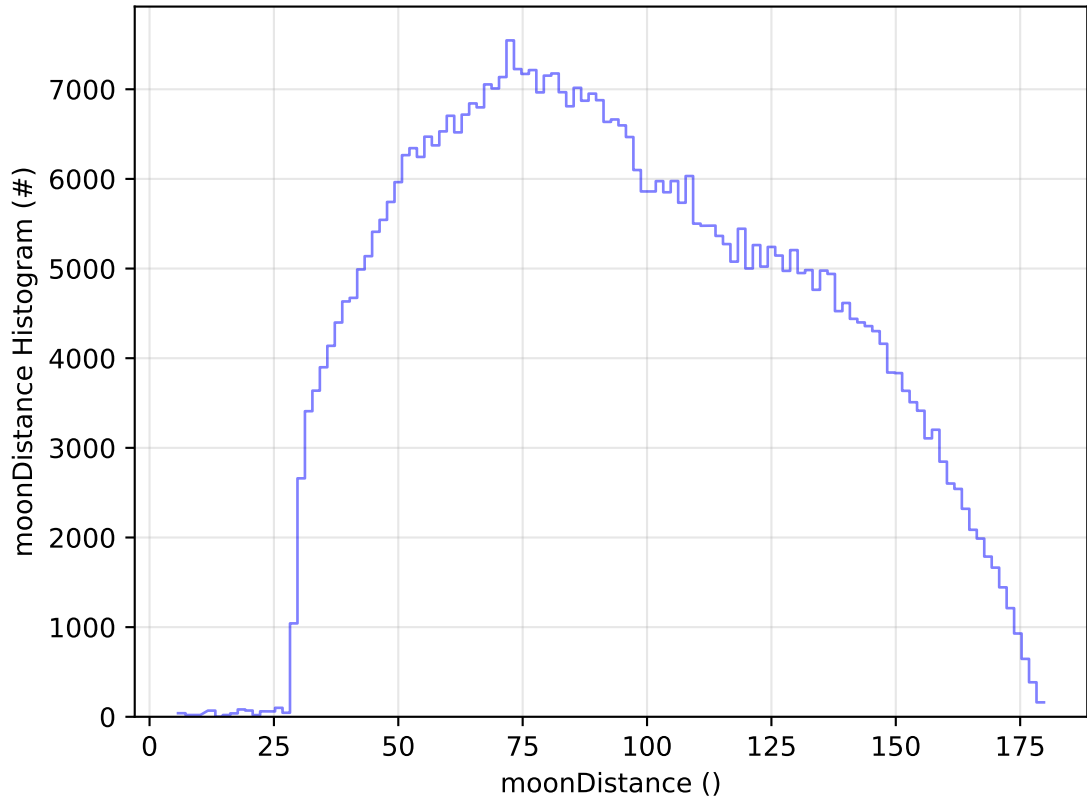
roll_uniform_early_half_mjdp0_v3.4_10yrs All sky i band: moonDistance Histogram
