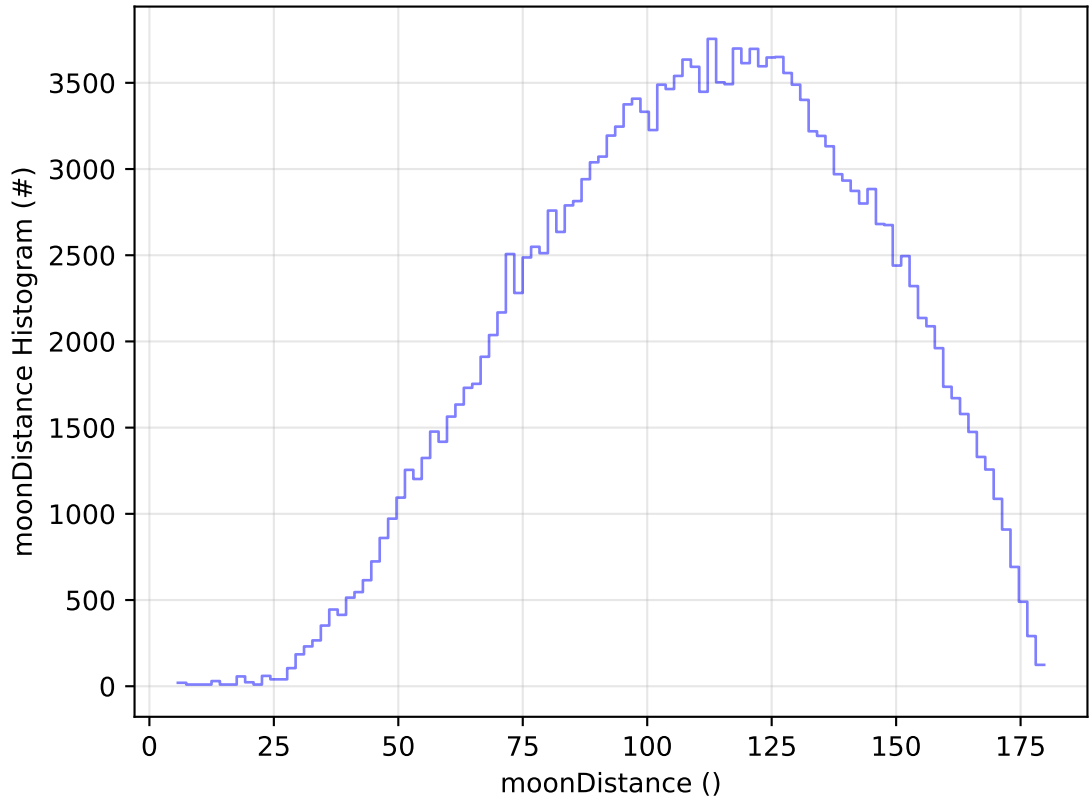
roll_uniform_early_half_mjdp0_v3.4_10yrs All sky g band: moonDistance Histogram
