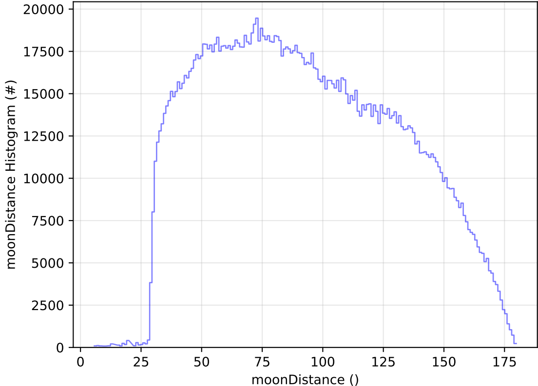
roll_uniform_early_half_mjdp0_v3.4_10yrs All sky all bands: moonDistance Histogram
