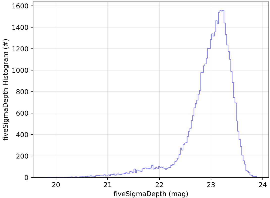
roll_uniform_early_half_mjdp0_v3.4_10yrs Yr 1 z band: fiveSigmaDepth Histogram
