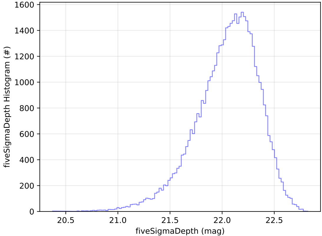
roll_uniform_early_half_mjdp0_v3.4_10yrs Yr 1 y band: fiveSigmaDepth Histogram
