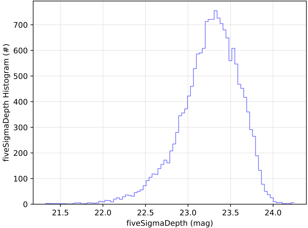
roll_uniform_early_half_mjdp0_v3.4_10yrs Yr 1 u band: fiveSigmaDepth Histogram
