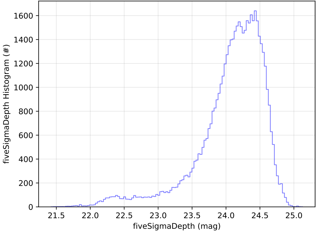
roll_uniform_early_half_mjdp0_v3.4_10yrs Yr 1 r band: fiveSigmaDepth Histogram
