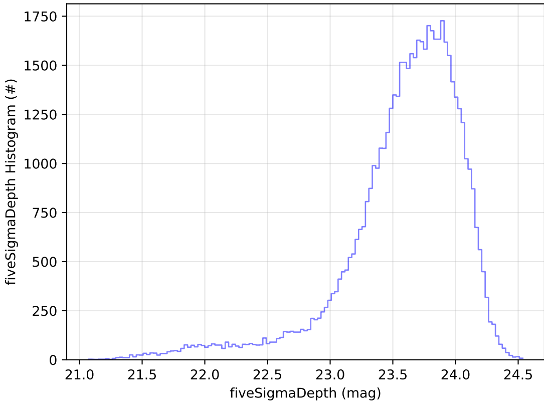
roll_uniform_early_half_mjdp0_v3.4_10yrs Yr 1 i band: fiveSigmaDepth Histogram
