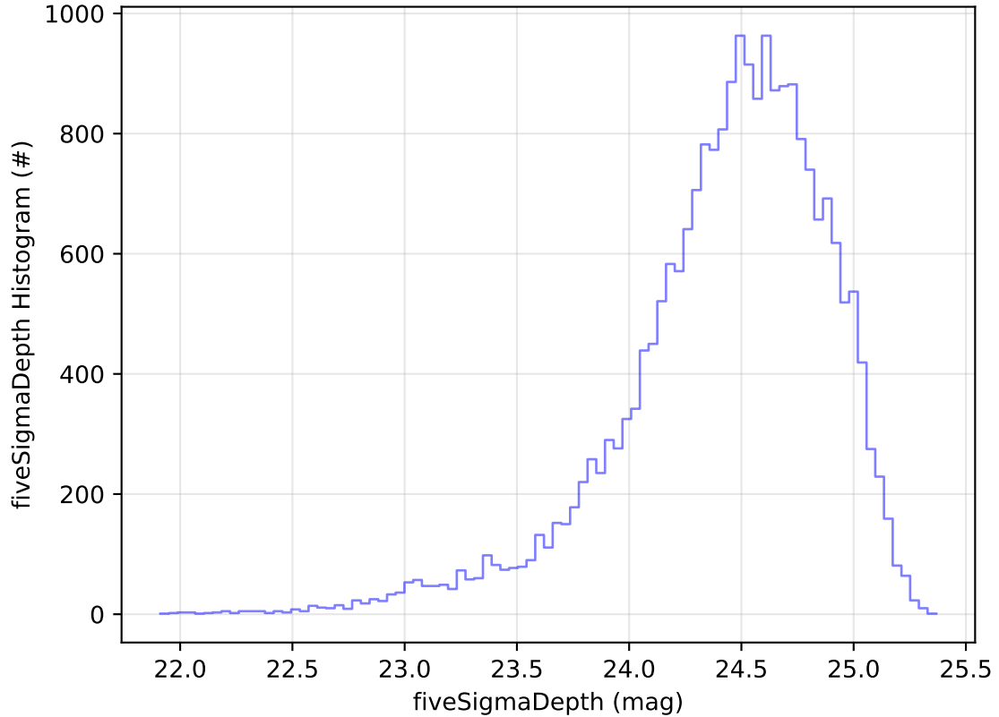
roll_uniform_early_half_mjdp0_v3.4_10yrs Yr 1 g band: fiveSigmaDepth Histogram
