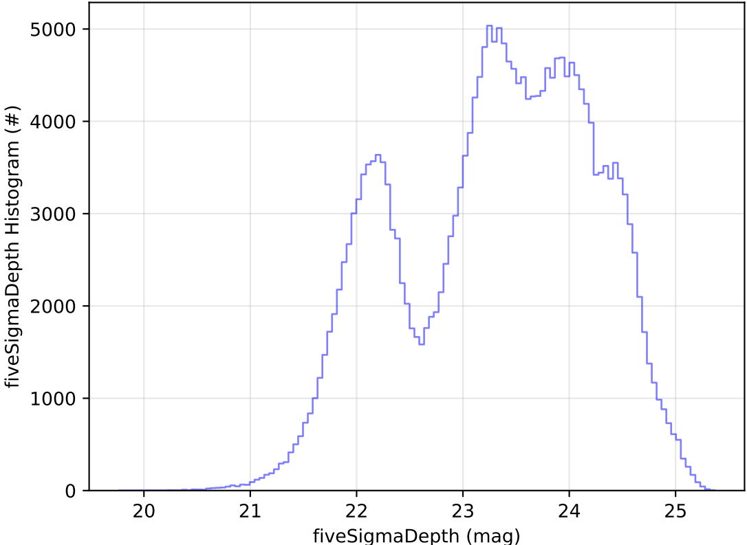
roll_uniform_early_half_mjdp0_v3.4_10yrs Yr 1 all bands: fiveSigmaDepth Histogram
