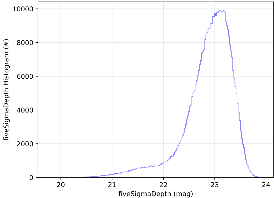
roll_uniform_early_half_mjdp0_v3.4_10yrs WFD z band: fiveSigmaDepth Histogram
