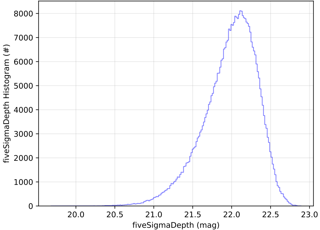
roll_uniform_early_half_mjdp0_v3.4_10yrs WFD y band: fiveSigmaDepth Histogram
