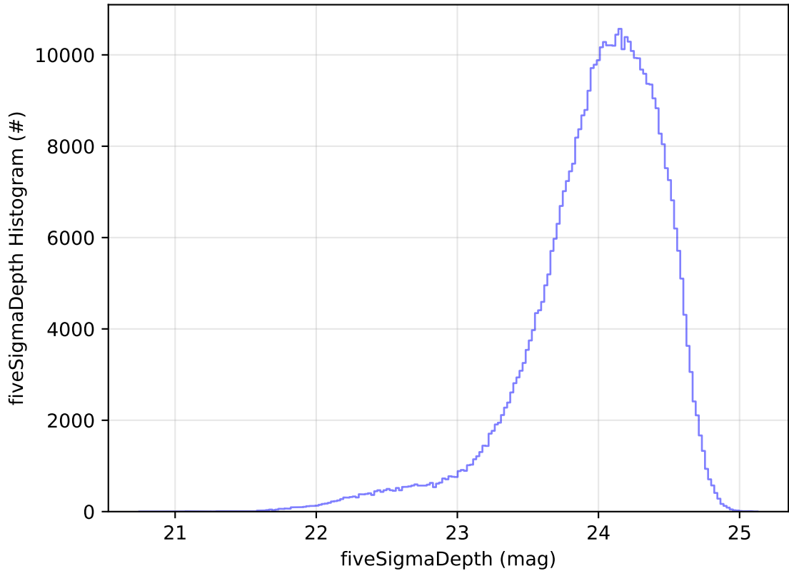
roll_uniform_early_half_mjdp0_v3.4_10yrs WFD r band: fiveSigmaDepth Histogram
