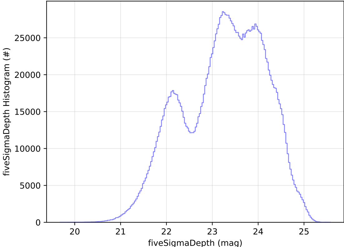
roll_uniform_early_half_mjdp0_v3.4_10yrs WFD all bands: fiveSigmaDepth Histogram
