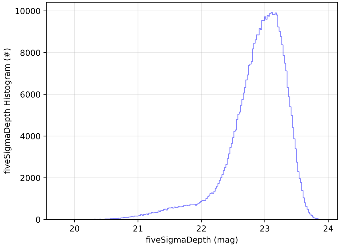
roll_uniform_early_half_mjdp0_v3.4_10yrs All sky z band: fiveSigmaDepth Histogram
