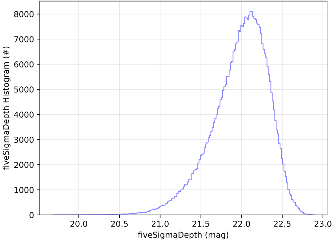
roll_uniform_early_half_mjdp0_v3.4_10yrs All sky y band: fiveSigmaDepth Histogram
