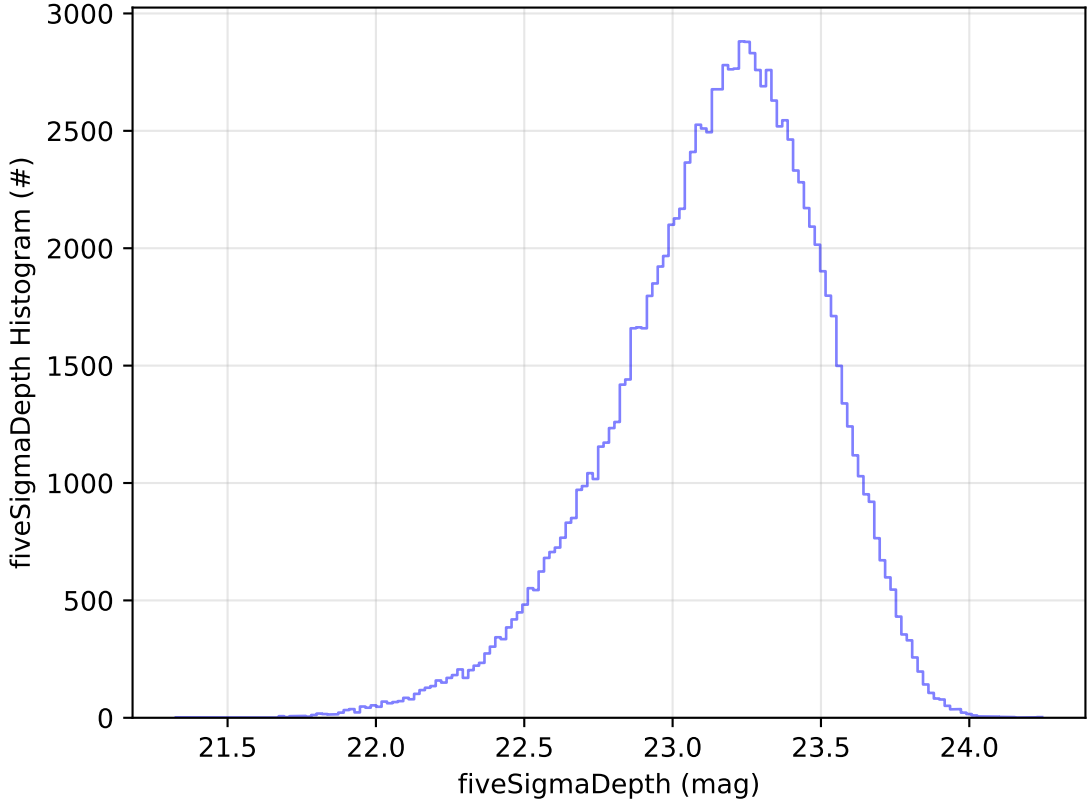
roll_uniform_early_half_mjdp0_v3.4_10yrs All sky u band: fiveSigmaDepth Histogram
