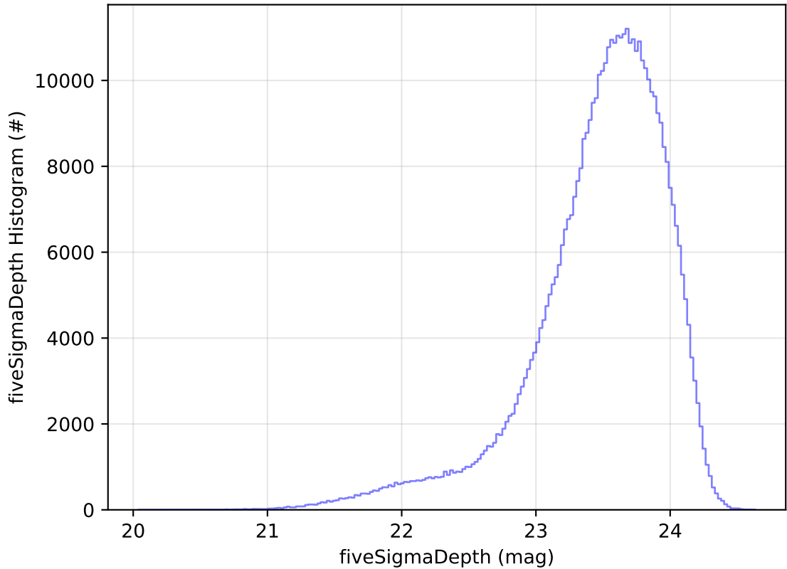
roll_uniform_early_half_mjdp0_v3.4_10yrs All sky i band: fiveSigmaDepth Histogram
