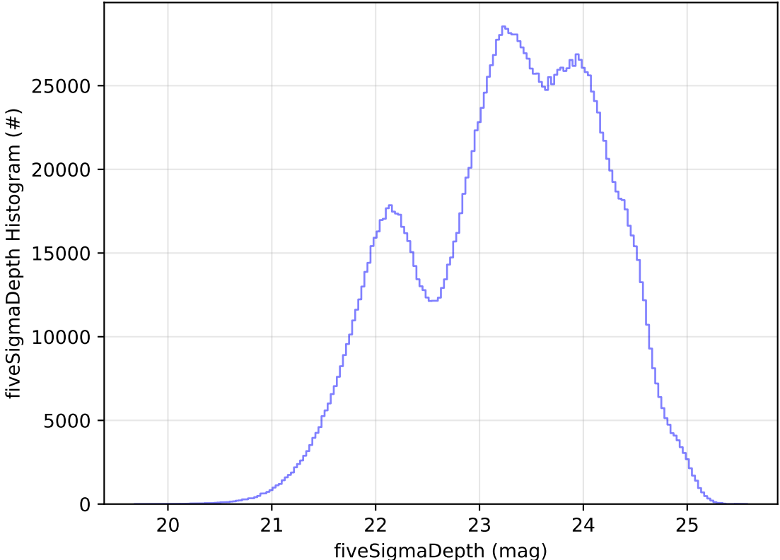
roll_uniform_early_half_mjdp0_v3.4_10yrs All sky all bands: fiveSigmaDepth Histogram
