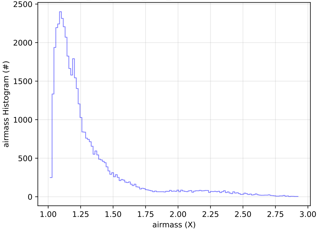
roll_uniform_early_half_mjdp0_v3.4_10yrs Yr 1 z band: airmass Histogram
