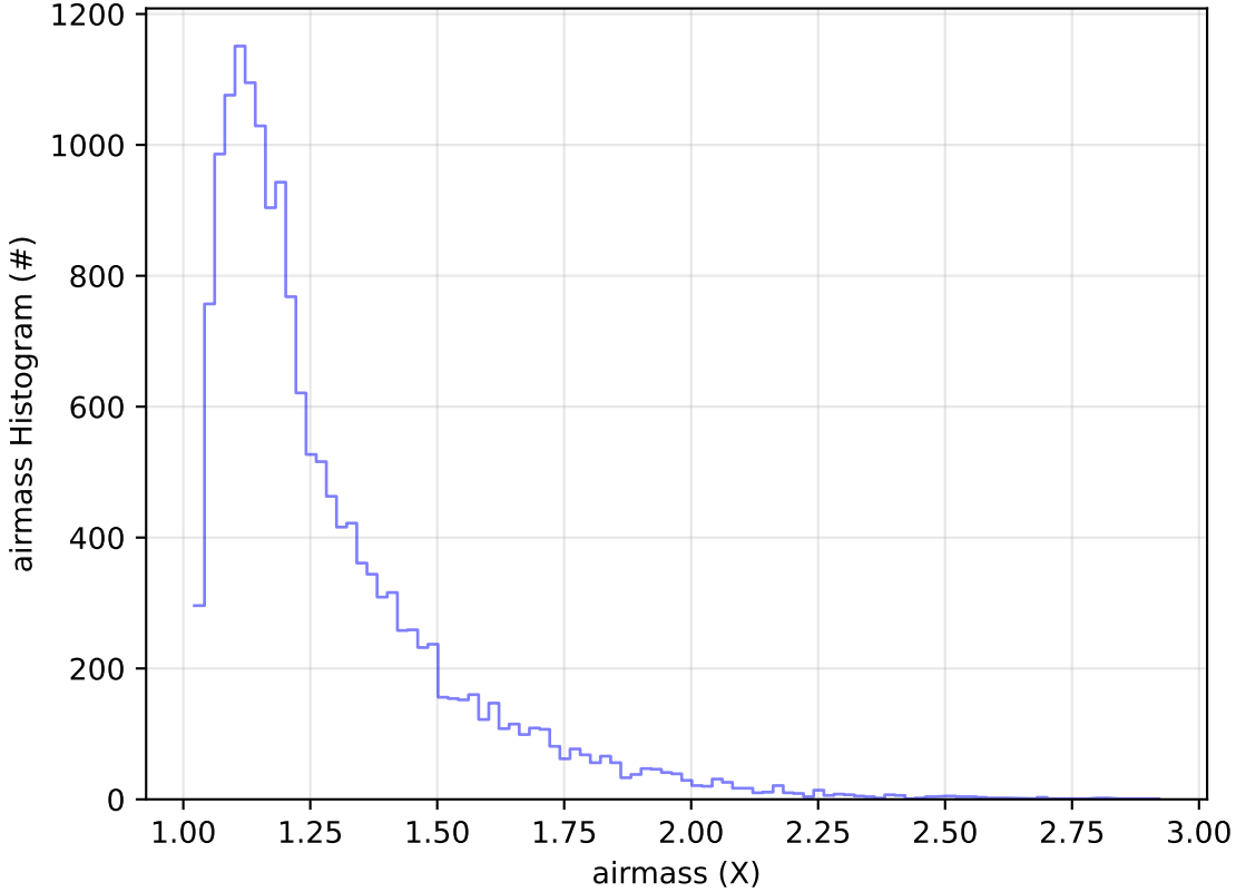
roll_uniform_early_half_mjdp0_v3.4_10yrs Yr 1 u band: airmass Histogram
