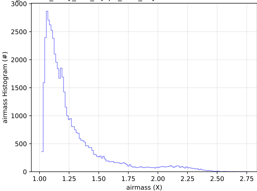
roll_uniform_early_half_mjdp0_v3.4_10yrs Yr 1 r band: airmass Histogram
