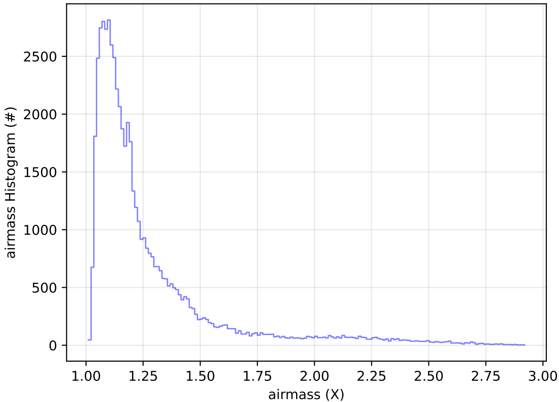
roll_uniform_early_half_mjdp0_v3.4_10yrs Yr 1 i band: airmass Histogram
